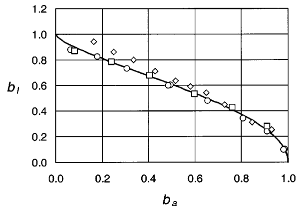
FIG. 3. Stability limits for noncylindrical volume bridges subject to steady nonaxisymmetric acceleration in terms of the dimensionless reduced axial and lateral Bond numbers, b_a and b_l . Symbols denote the calculated results using SURFACE EVOLVER, according to the following key: V=1.1 (circle), V=1.2 (rectangle), V=1.3 (rhomb), and the solid line is Eq. (4).
